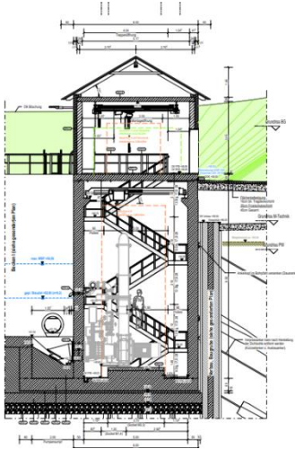
Autodesk Revit
